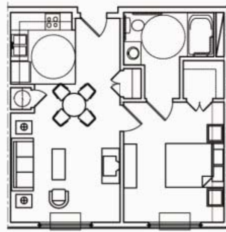
2 HANDICAPPED UNITS - ONE BEDROOM WITH ACCESSIBLE TUB (625 SF)
