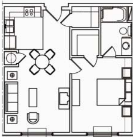
57 UNITS - ONE BEDROOM (625 SF)
